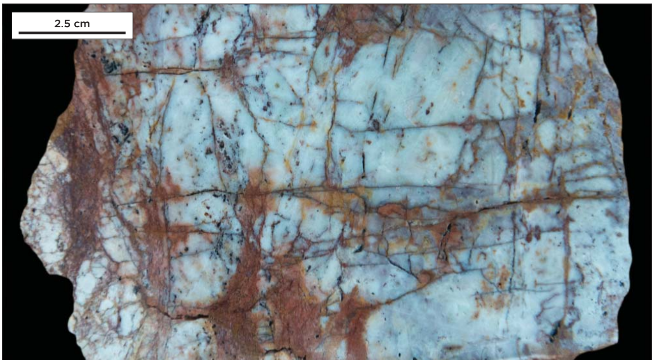
Figure 22: Fracture oxidized, massive, light grey green cryptocrystalline quartz, with fine gossanous vughs after sulphides. EAL sample ER01427 which assayed 7.28 g/t Au and 0.35 oz/t Ag.
